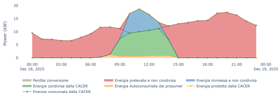
Flussi energetici - 2025-12-18 - CACER
